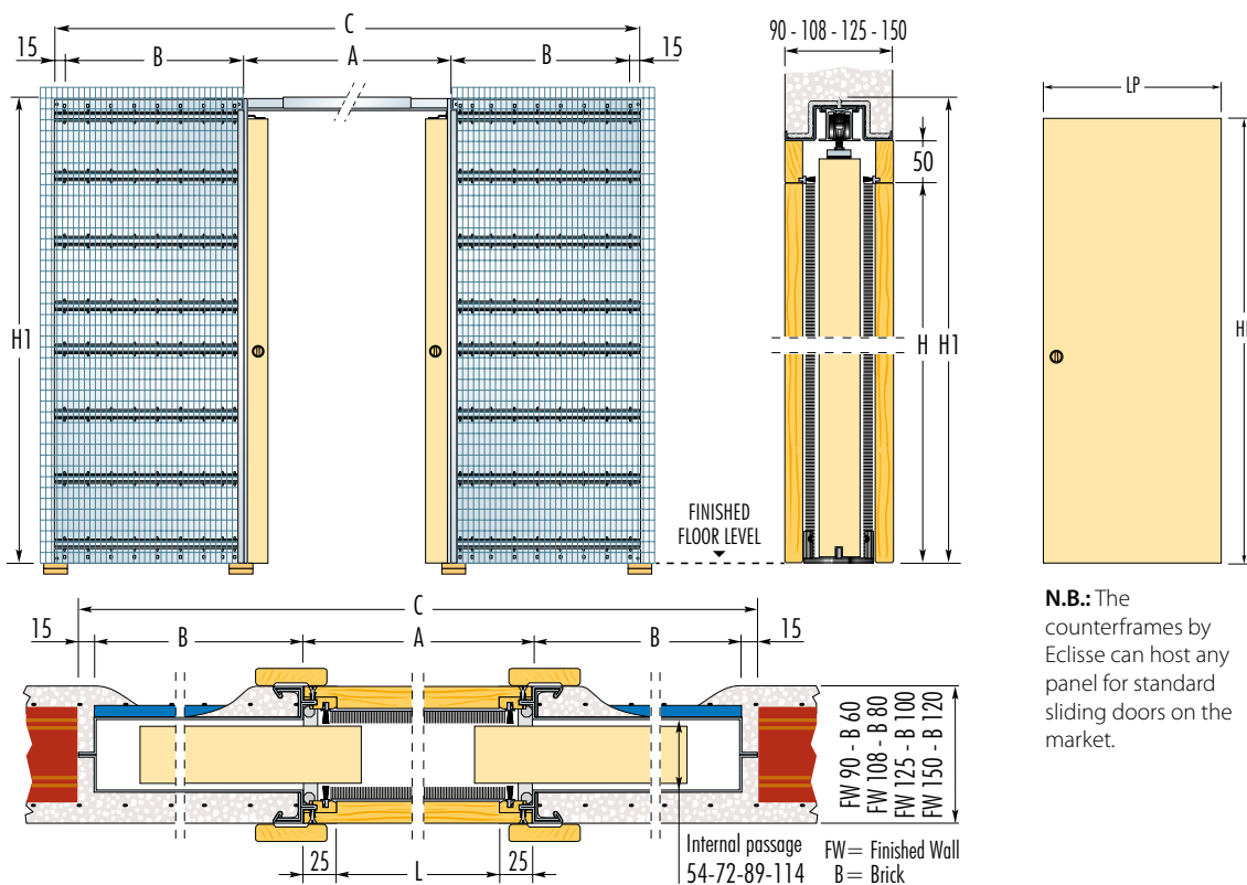
FRAMES FOR DOUBLE DOORS - Measures related to Italian standards, other dimensions available
